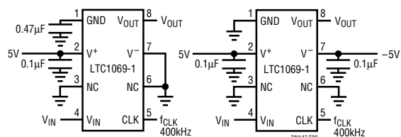
Figure 2. Single 5V or Dual \pm 5V Supply 4kHz Elliptic Lowpass Filter
