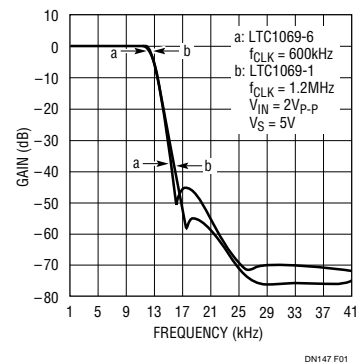
Figure 1. Amplitude Response Comparison: LTC1069-1 vs LTC1069-6
