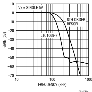
Figure 4. Frequency Response
